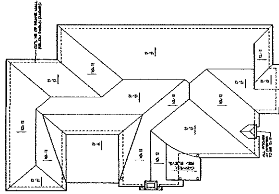
② ROOF PLAN 1/8" = 1'-0"
